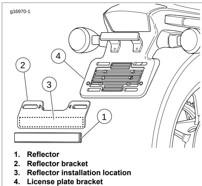
Figure 1. Reflector
