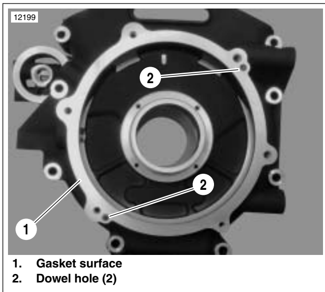
Figure 16. Crankcase
