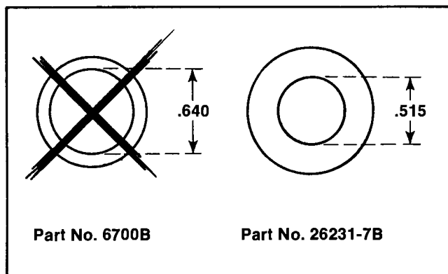
Figure 1. Drain Plug Washer
