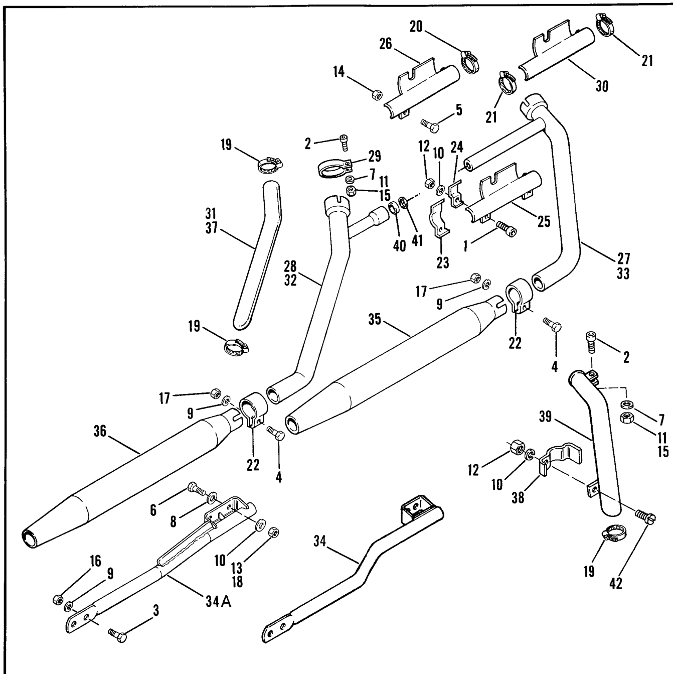
Figure 2. XL Exhaust System — 1980 and Later
