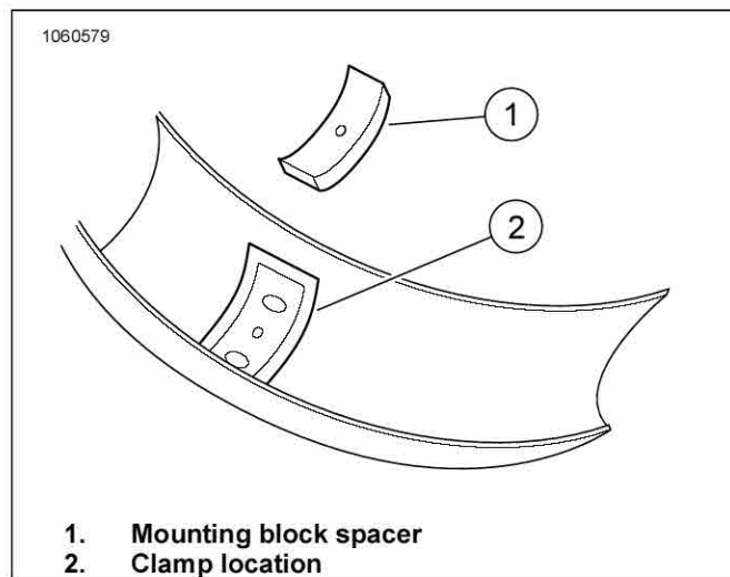
Figure 2. Mounting Block Spacer
