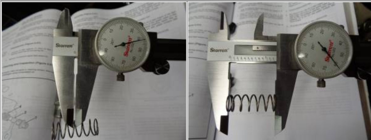
1992-up Check Ball Spring Dims (used and working spring)
